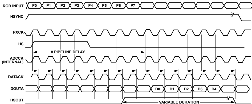
Figure 16. Single-Port Mode
