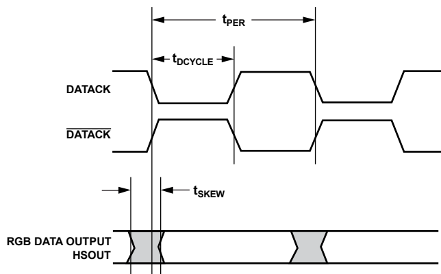
Figure 15. Output Timing
