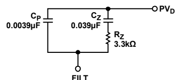
Figure 9. PLL Loop Filter Detail
