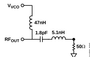
Figure 22. Optimum ADF4360-4 Output Stage
