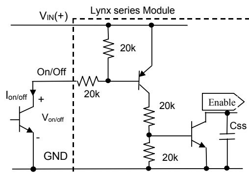
Figure 28. Remote On/Off Implementation.
