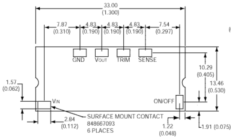
BOTTOM VIEW OF BOARD
