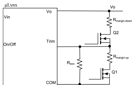
Figure 31. Circuit Configuration for margining Output voltage.
