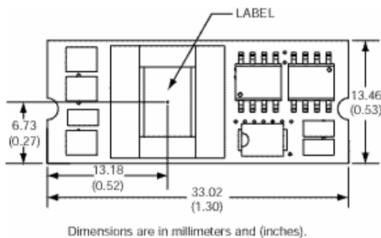
Figure 35. Pick and Place Location.
