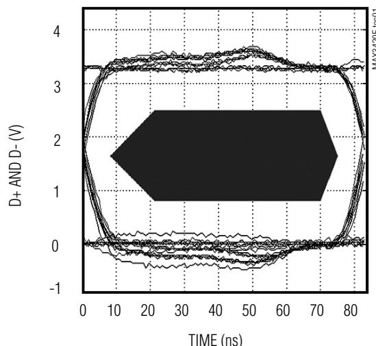
EYE DIAGRAM
