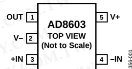
Figure 1. 5-Lead TSOT (UJ Suffix)
