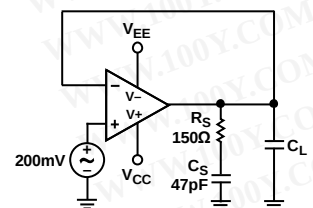
Figure 43. Snubber Network
