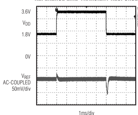
REFERENCE LINE-TRANSIENT RESPONSE
