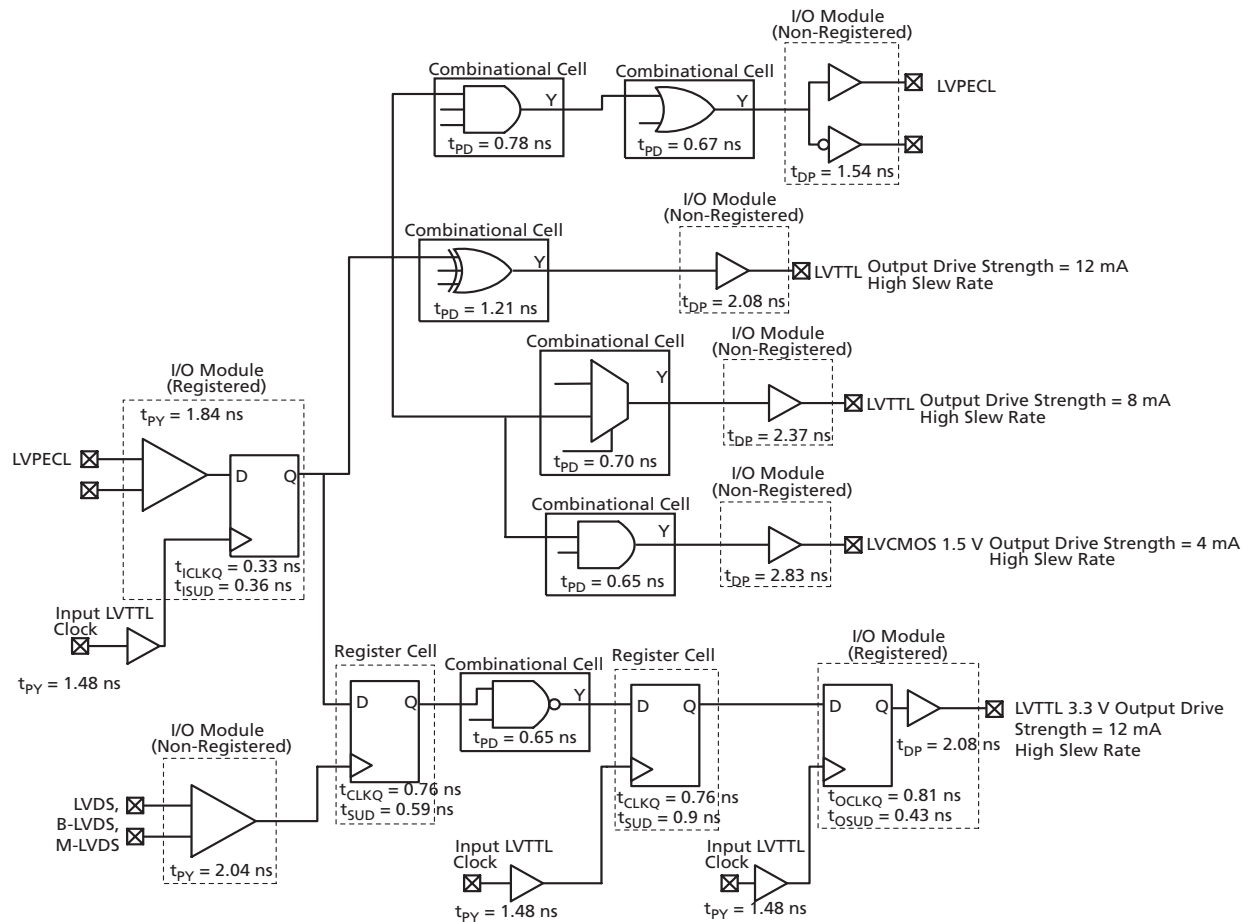
Figure 2-4 • Timing Model
