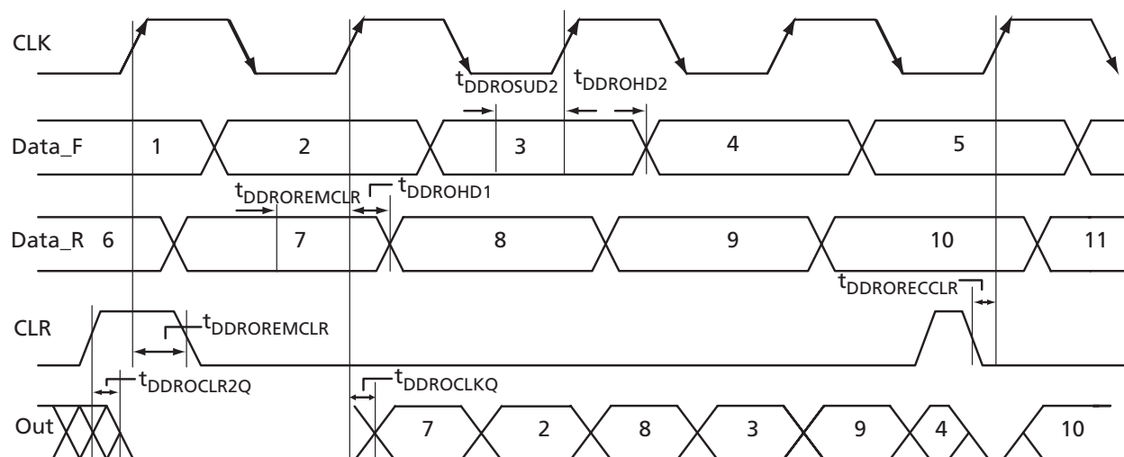
Figure 2-35 • Output DDR Timing Diagram
