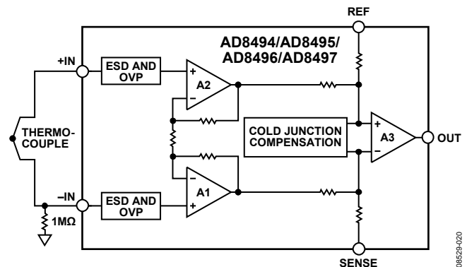
Figure 27. Block Diagram
