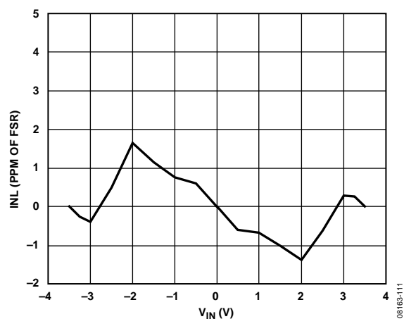
Figure 11. INL (Gain = 1)
