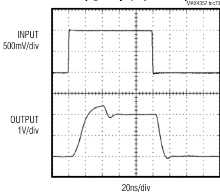
LARGE-SIGNAL PULSE RESPONSE WITH CAPACITIVE LOAD ( C_L = 30\text{pF} , A_V = +2\text{V/V} )
