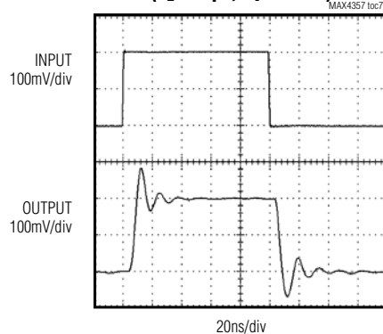
MEDIUM-SIGNAL PULSE RESPONSE WITH CAPACITIVE LOAD ( C_L = 30\text{pF} , A_V = +1\text{V/V} )
