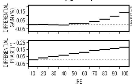
DIFFERENTIAL GAIN AND PHASE ( R_L = 1\text{k}\Omega )
