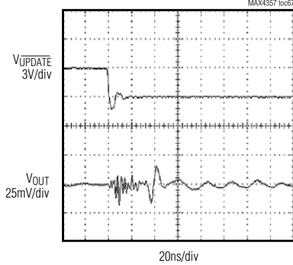
SWITCHING TRANSIENT GLITCH ( A_V = +1\text{V/V} )
