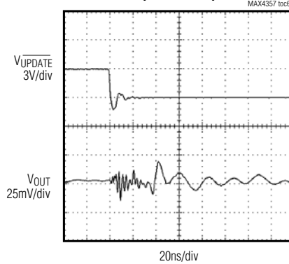
SWITCHING TRANSIENT GLITCH ( A_V = +2\text{V/V} )
