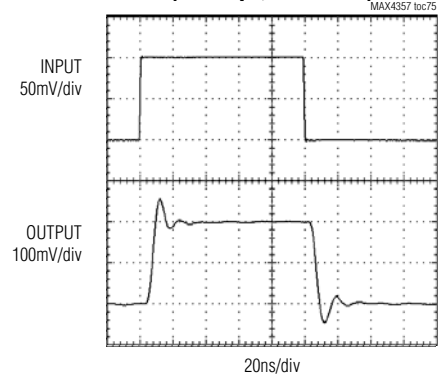
MEDIUM-SIGNAL PULSE RESPONSE WITH CAPACITIVE LOAD ( C_L = 30\text{pF} , A_V = +2\text{V/V} )
