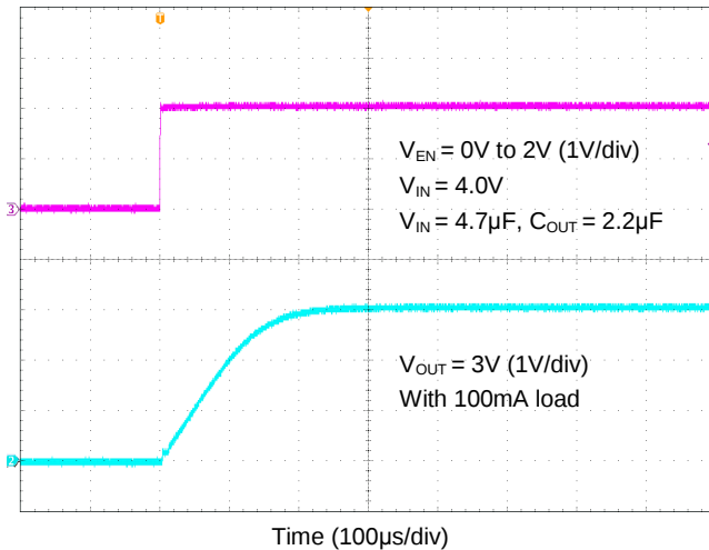
Start-up Time
