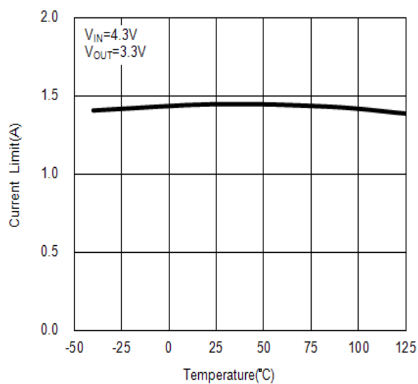
Current Limit vs Temperature
