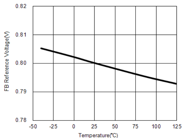
FB Reference Voltage vs Temperature
