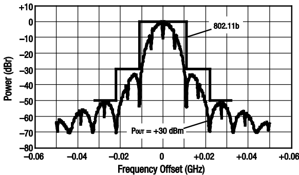
Figure 8. Spectral Mask (1 Mbps)
