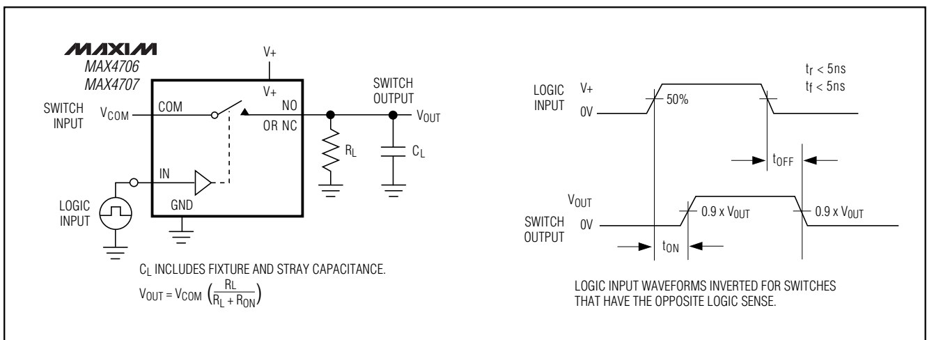
Figure 2. Switching Time
