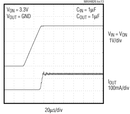
CURRENT-LIMIT RESPONSE
