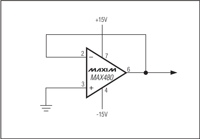
Figure 2. Burn-In Circuit
