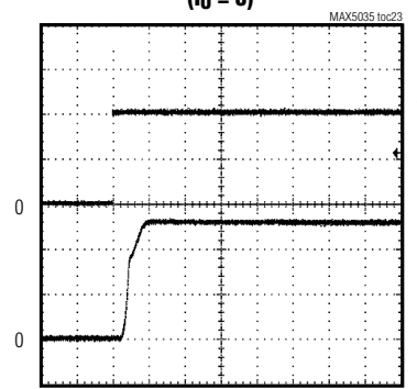
MAX5035DASA STARTUP WAVEFORM ( I_O = 0 )
