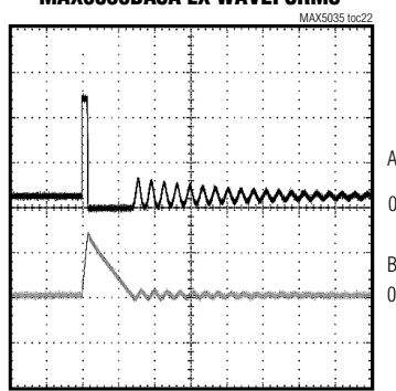
MAX5035DASA LX WAVEFORMS
