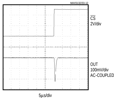
MAX5132 MAJOR CARRY TRANSITION
