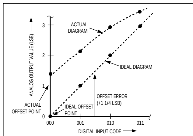
Figure 8c. Offset Error
