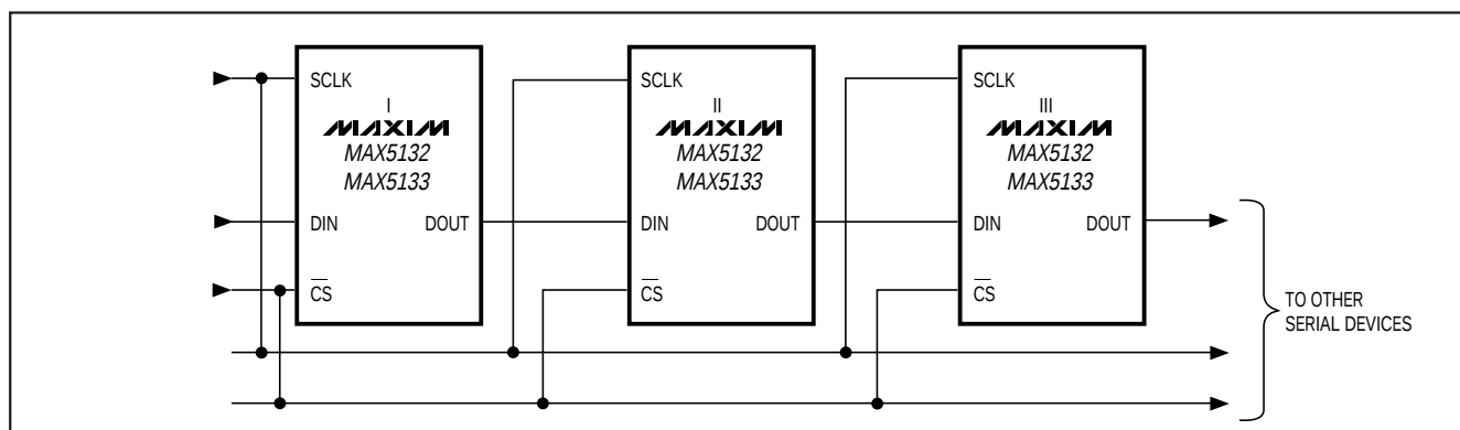
Figure 11. Daisy-Chaining Multiple Devices with the Digital I/Os DIN/DOUT
