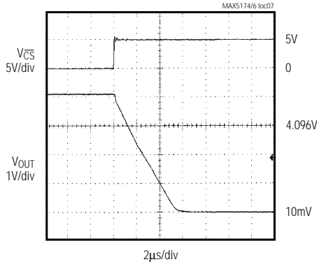
DYNAMIC RESPONSE
