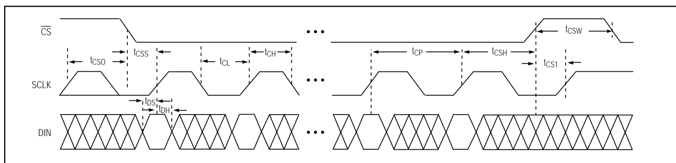
Figure 6. Detailed Serial-Interface Timing Diagram
