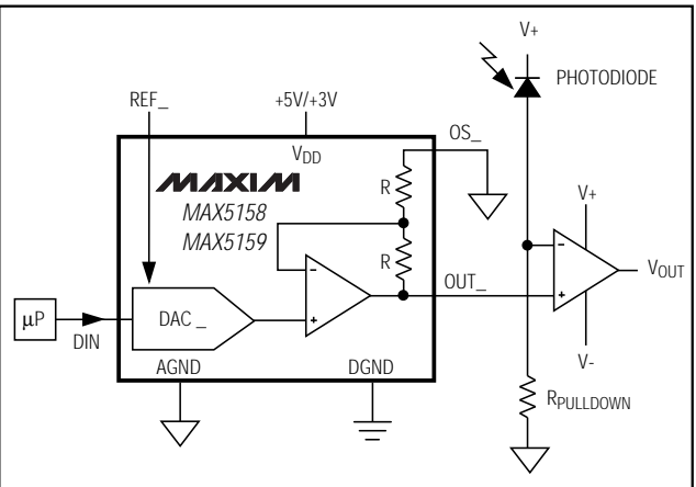
Figure 13. Digital Calibration
