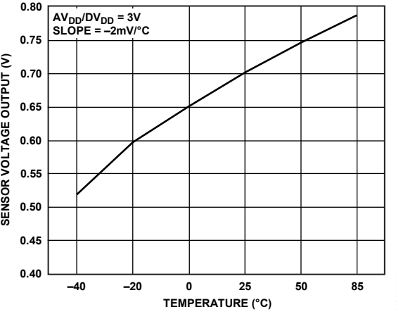
Figure 31. Typical Temperature Sensor Output vs. Temperature
