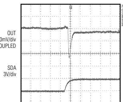
OUTPUT SETTLING 1LSB STEP DOWN
