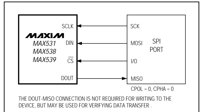
Figure 5. SPI/QSPI Connection
