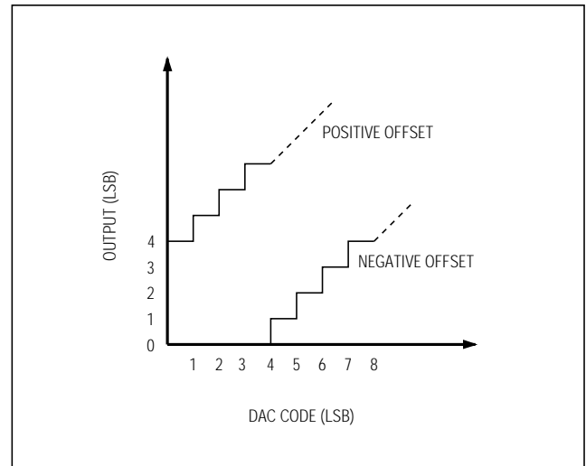
Figure 10. Single-Supply Offset
