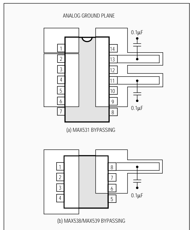
Figure 11. Power-Supply Bypassing
