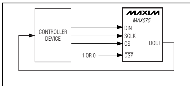
Figure 7. Stand-Alone Configuration
