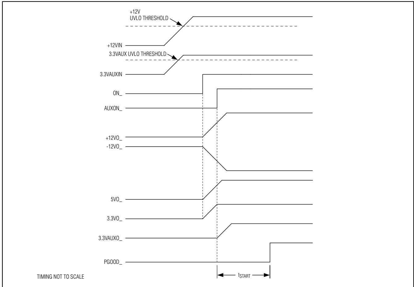
Figure 1. Startup Waveforms
