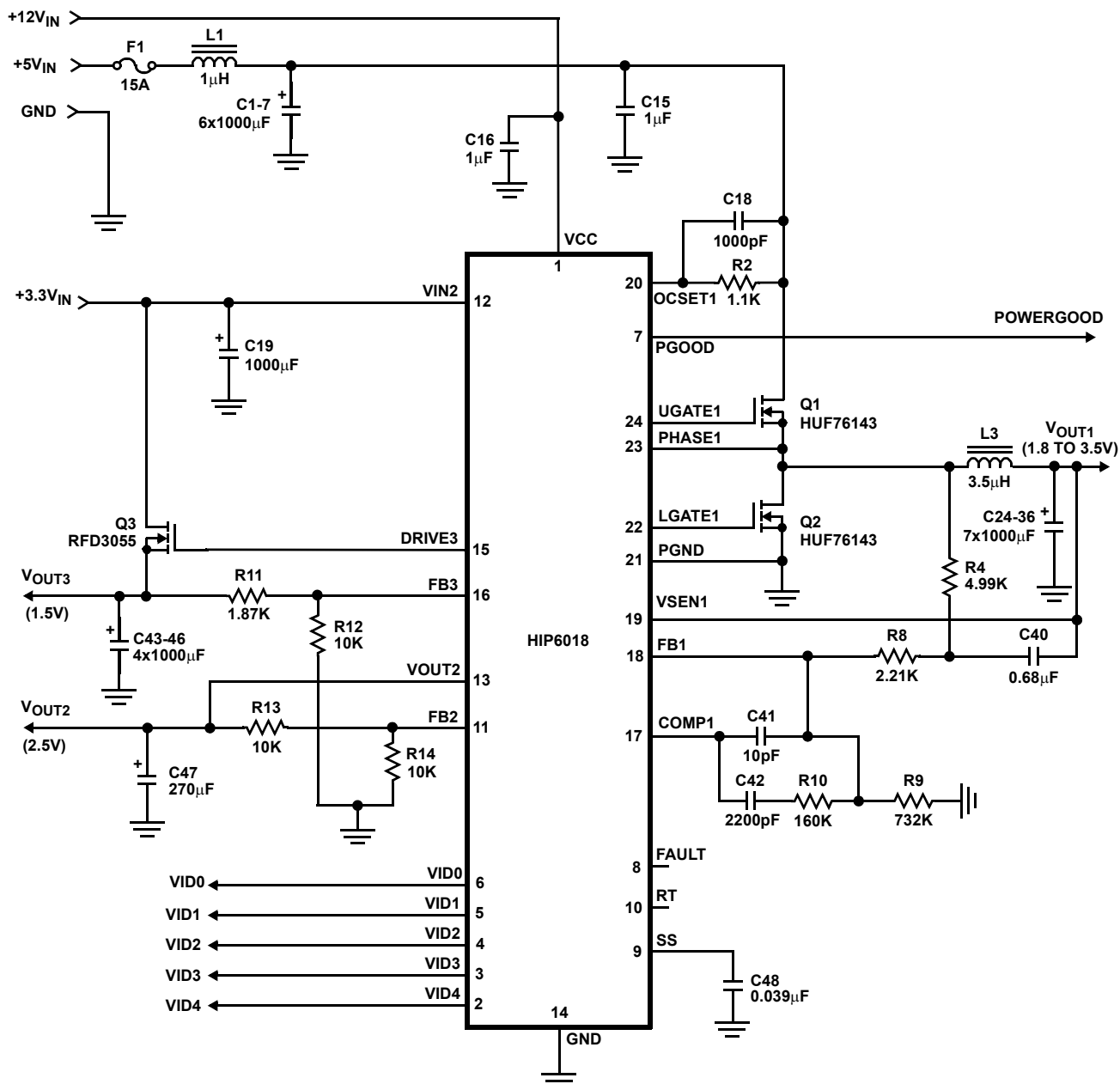
FIGURE 15. APPLICATION CIRCUIT
