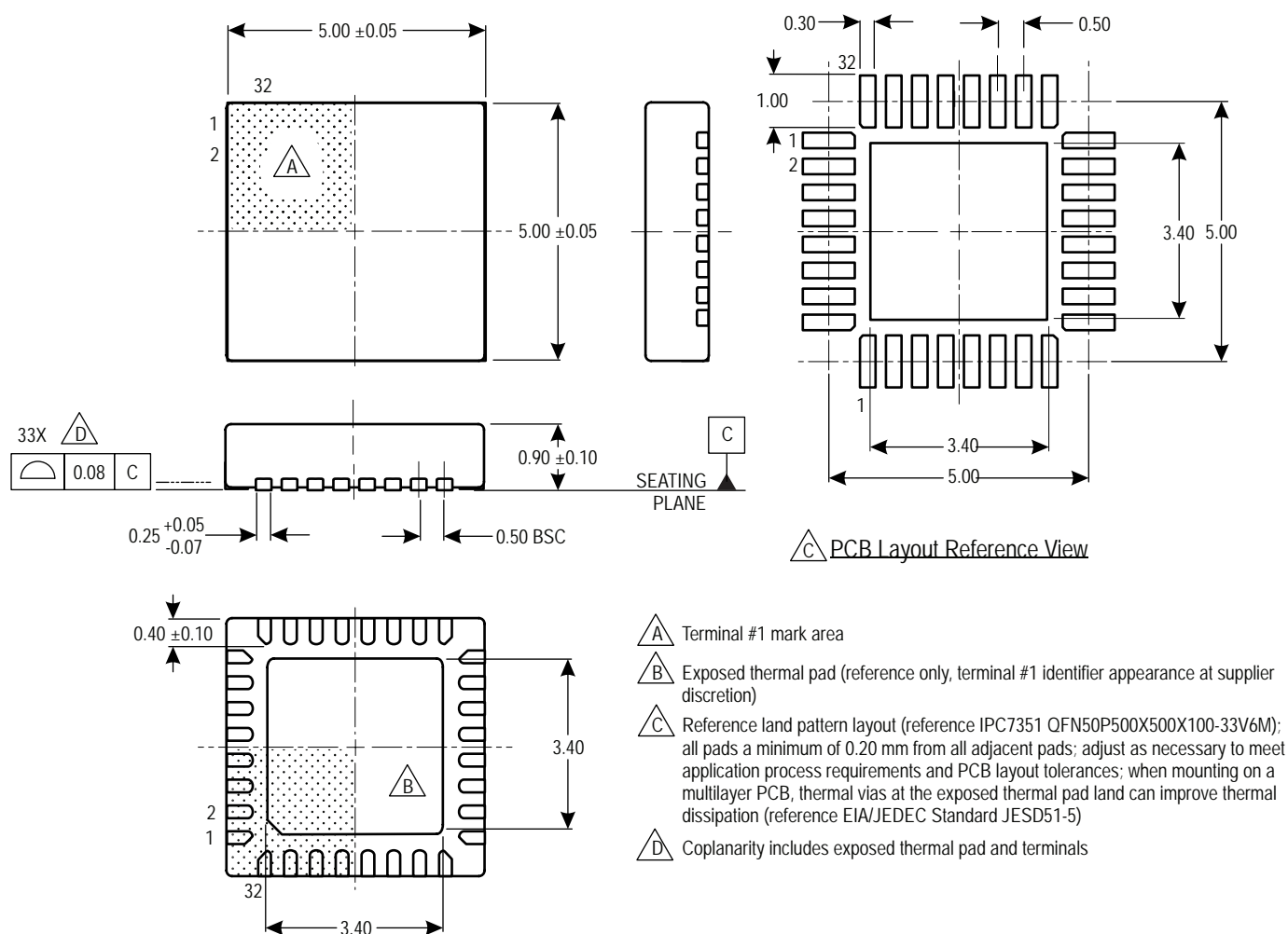
Figure 19: ET Package, 32-Pin QFN with Exposed Thermal Pad
