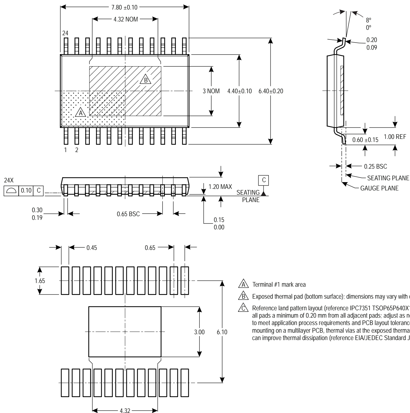
Figure 20: LP Package, 24-Pin TSSOP with Exposed Thermal Pad
