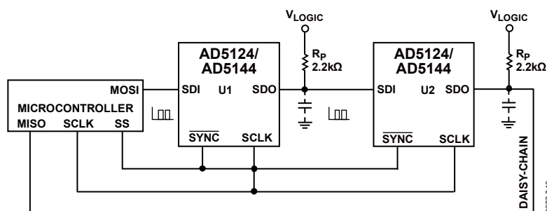
Figure 43. Daisy-Chain Configuration
