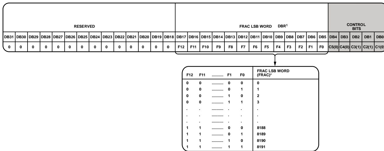
Figure 25. Register 6 (R6)
