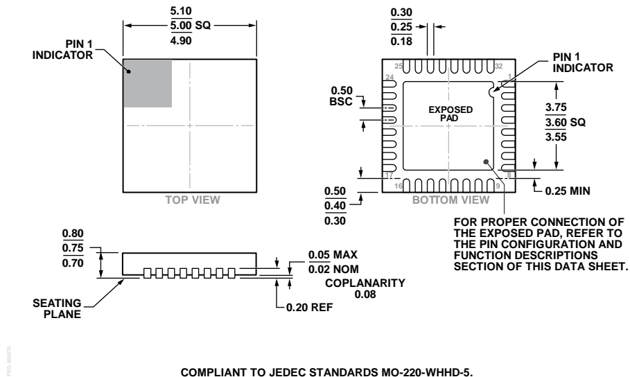
Figure 32. 32-Lead Lead Frame Chip Scale Package [LFCSP_WQ] 5 mm × 5 mm Body, Very Very Thin Quad (CP-32-12)
