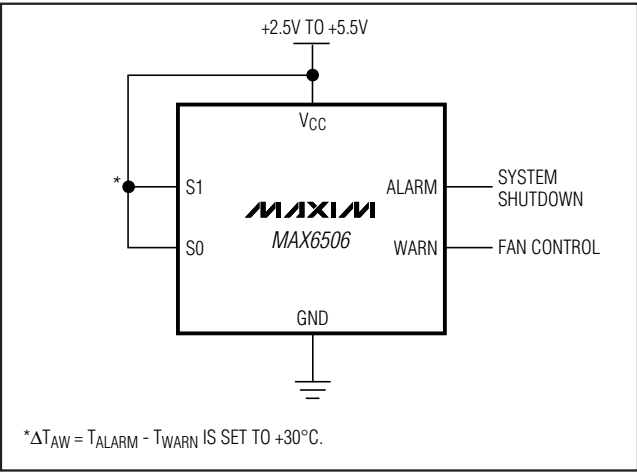
Figure 3. Low-Power, High-Reliability, Fail-Safe Temperature Monitor
