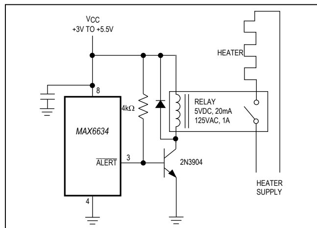
Figure 10. Simple Thermostat
