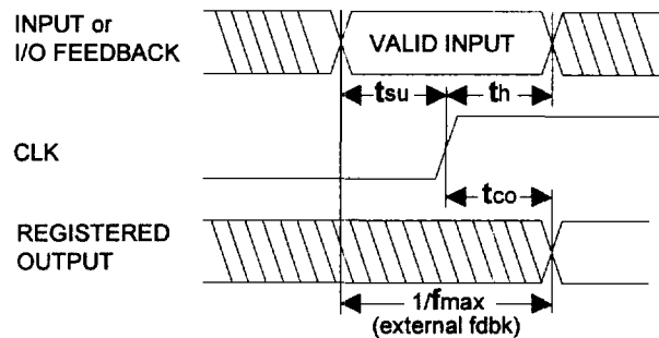
Registered Output
