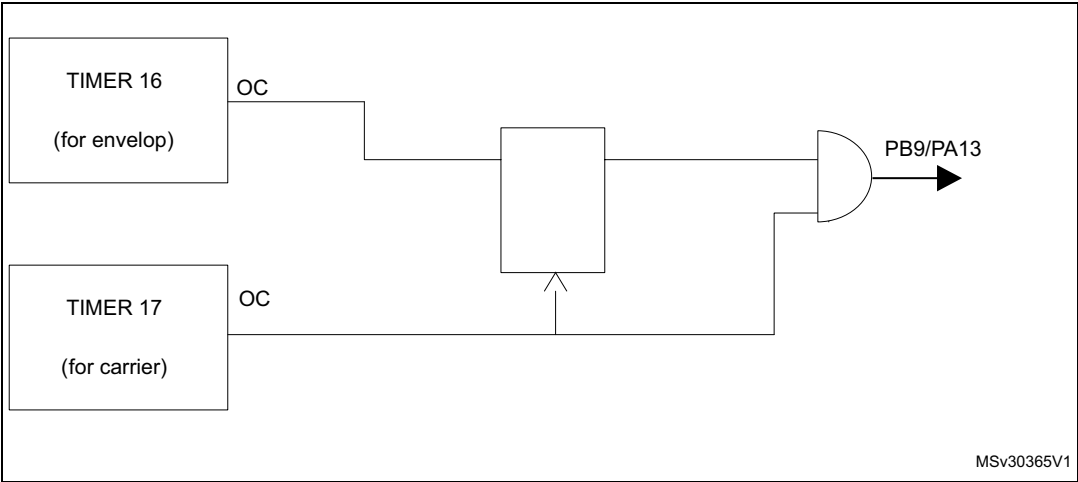
Figure 3. Infrared transmitter
