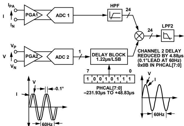
Figure 59. Phase Calibration
