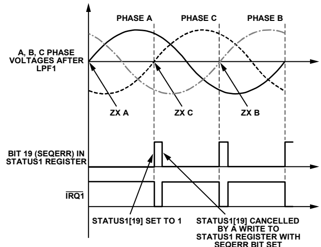
Figure 64. SEQERR Bit Set to 1 When Phase A Voltage Is Followed by Phase C Voltage
