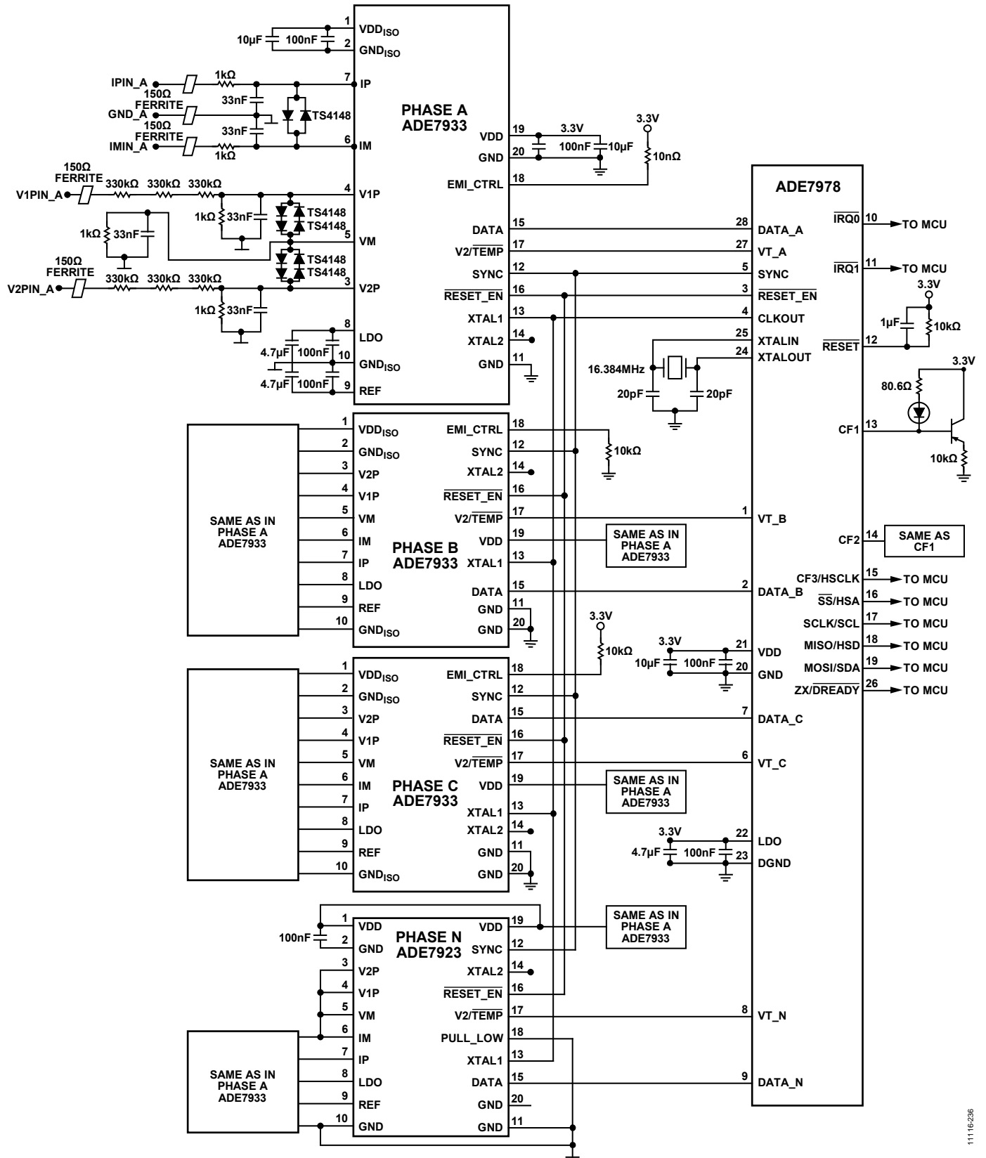
Figure 42. Test Circuit
