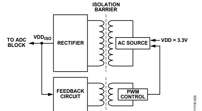
Figure 103. Isolated DC-to-DC Converter Block Diagram
