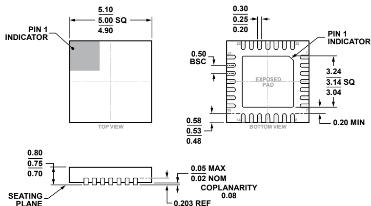
Figure 138. 28-Lead Lead Frame Chip Scale Package [LFCSP_WQ] 5 mm × 5 mm Body and 0.75 mm Package Height (CP-28-10)
