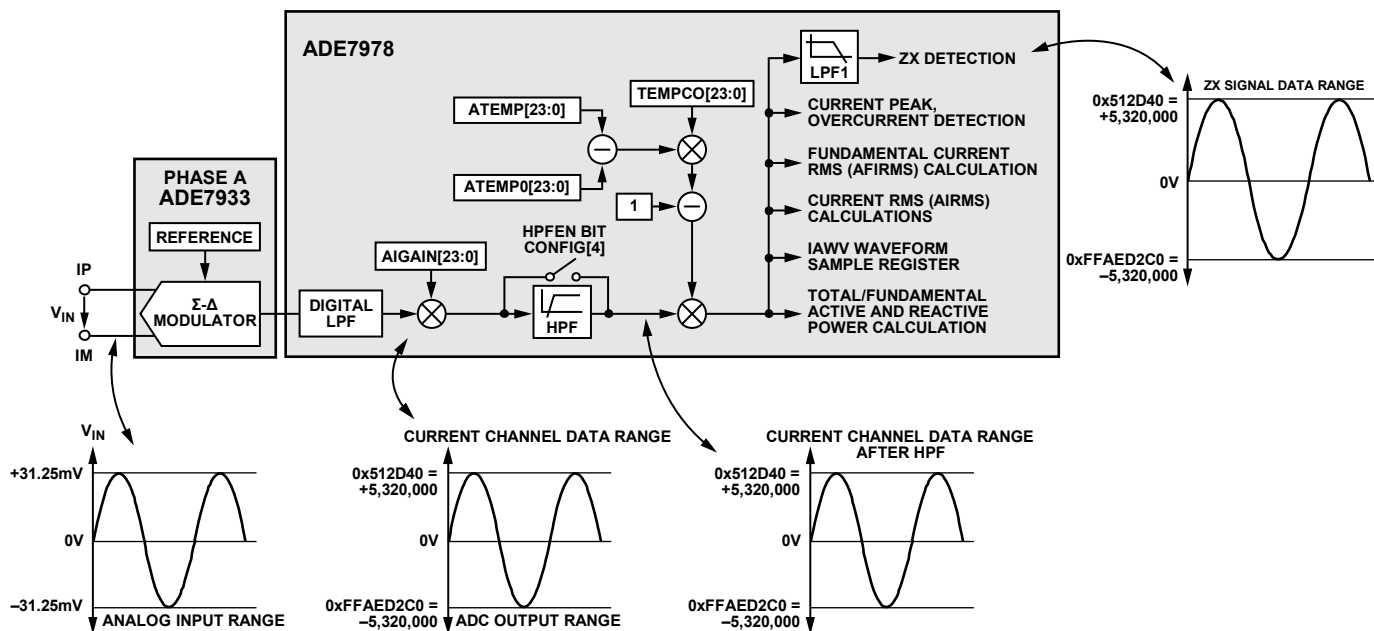
Figure 50. Phase A Current Channel Signal Path
