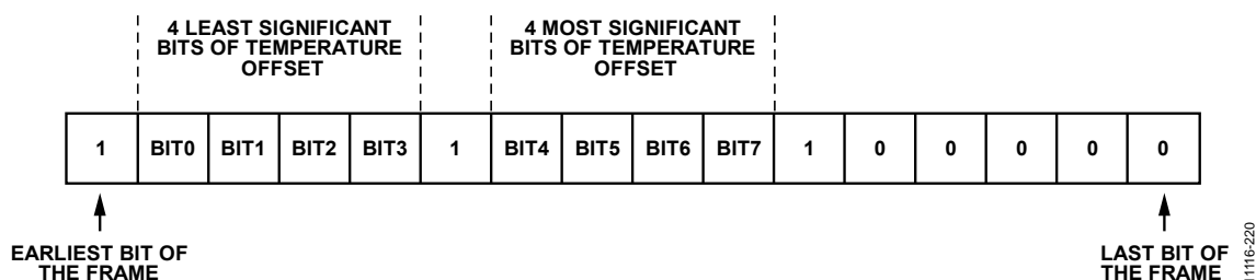
Figure 116. Temperature Offset Bit Stream Communication
