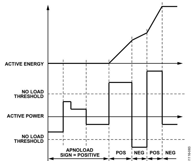
Figure 97. Active Power Absolute Accumulation Mode
