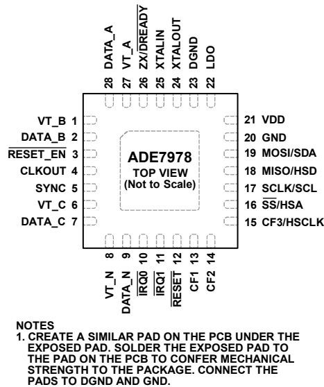
Figure 11. Pin Configuration, ADE7978
