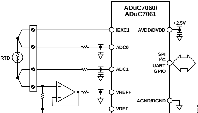
Figure 20. Example of an RTD Interface Circuit
