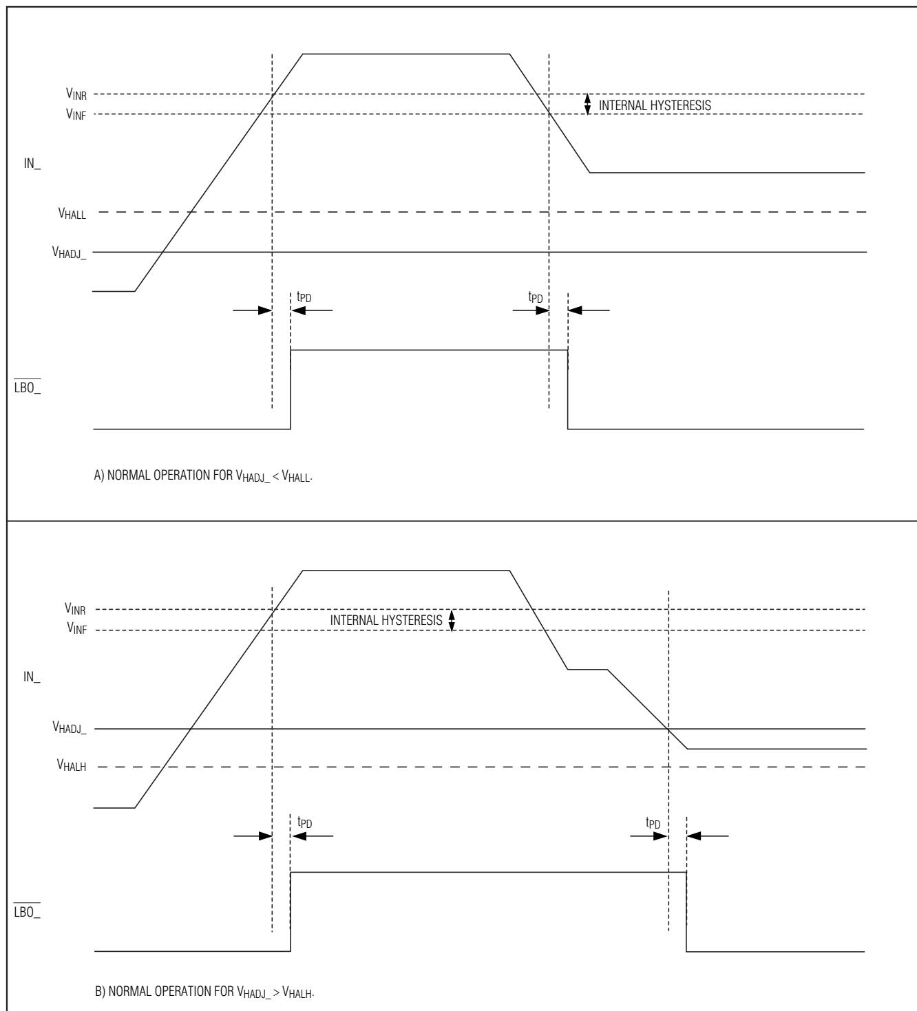
Figure 4. MAX6782-MAX6785 Timing
