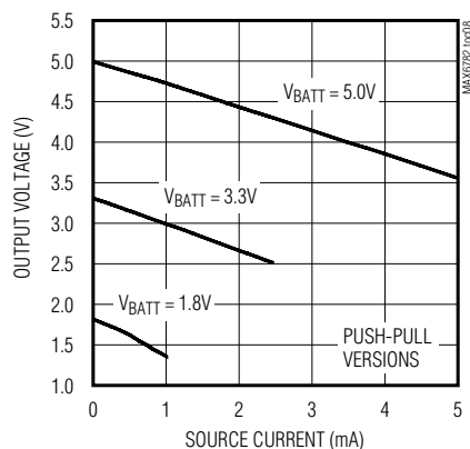
LBO OUTPUT VOLTAGE HIGH vs. SOURCE CURRENT
