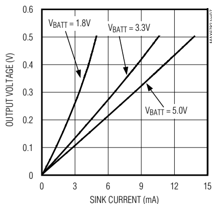
LBO OUTPUT VOLTAGE LOW vs. SINK CURRENT
