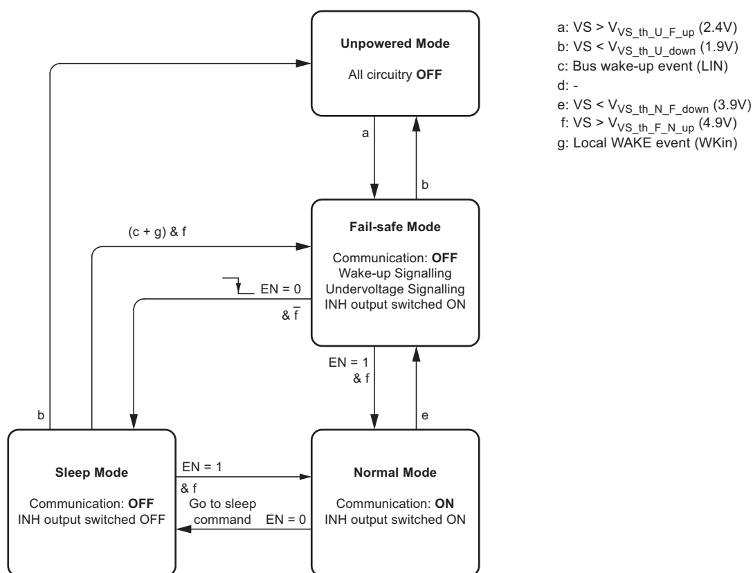
Figure 4-1. Operating Modes
