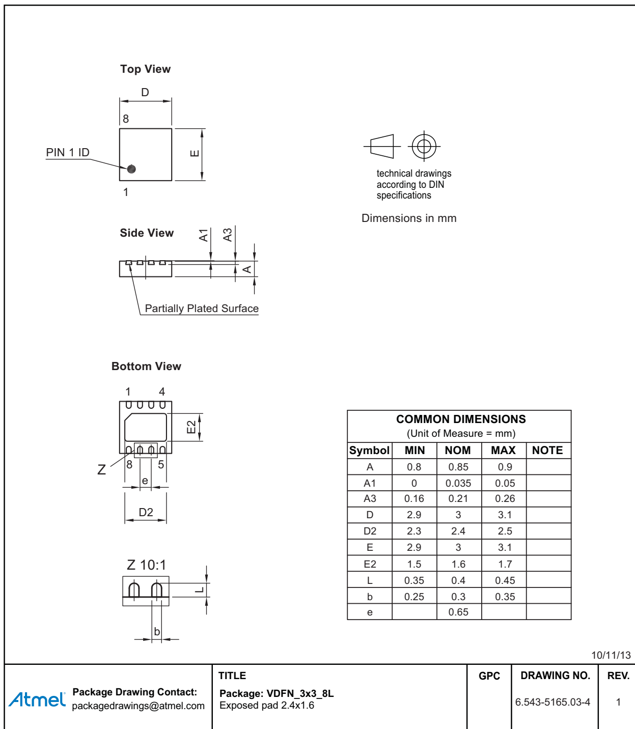
Figure 11-1. DFN8
