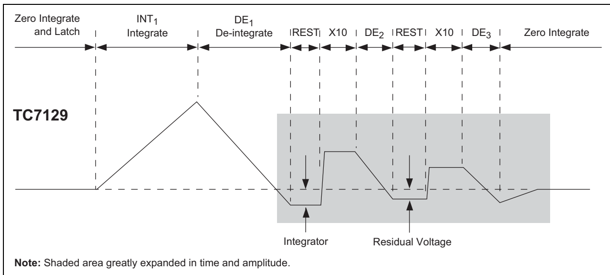
Figure 4-10: Integration Waveform.
