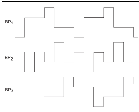
Figure 4-17: Backplane Waveforms.
