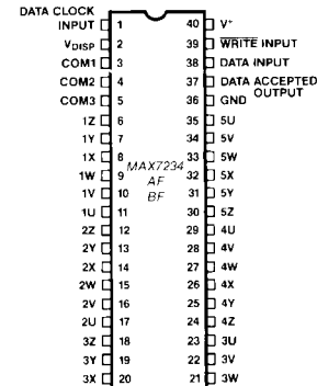
40 Lead DIP
