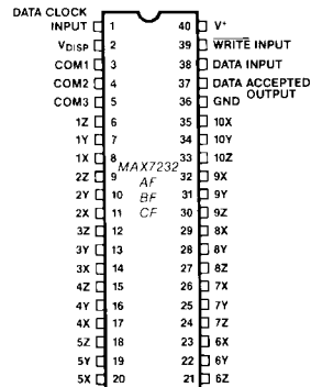
40 Lead DIP
