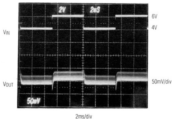
LINE-TRANSIENT RESPONSE
