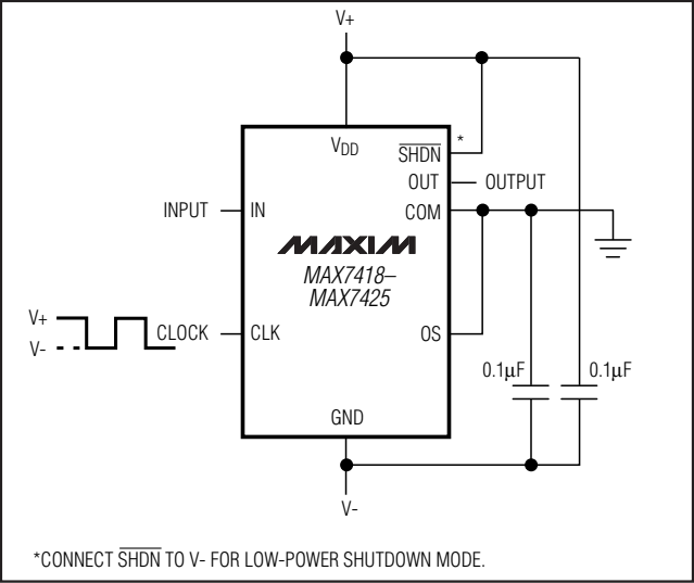
Figure 5. Dual-Supply Operation
