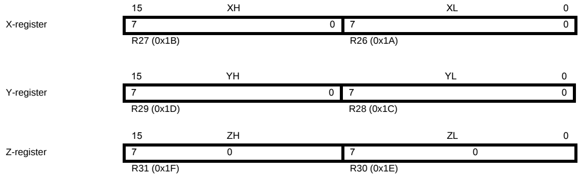
Figure 6-5. The X-, Y-, and Z-registers
