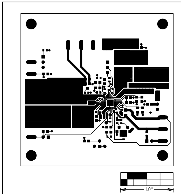
Figure 3. MAX8728 EV Kit PC Board Layout—Component Side
