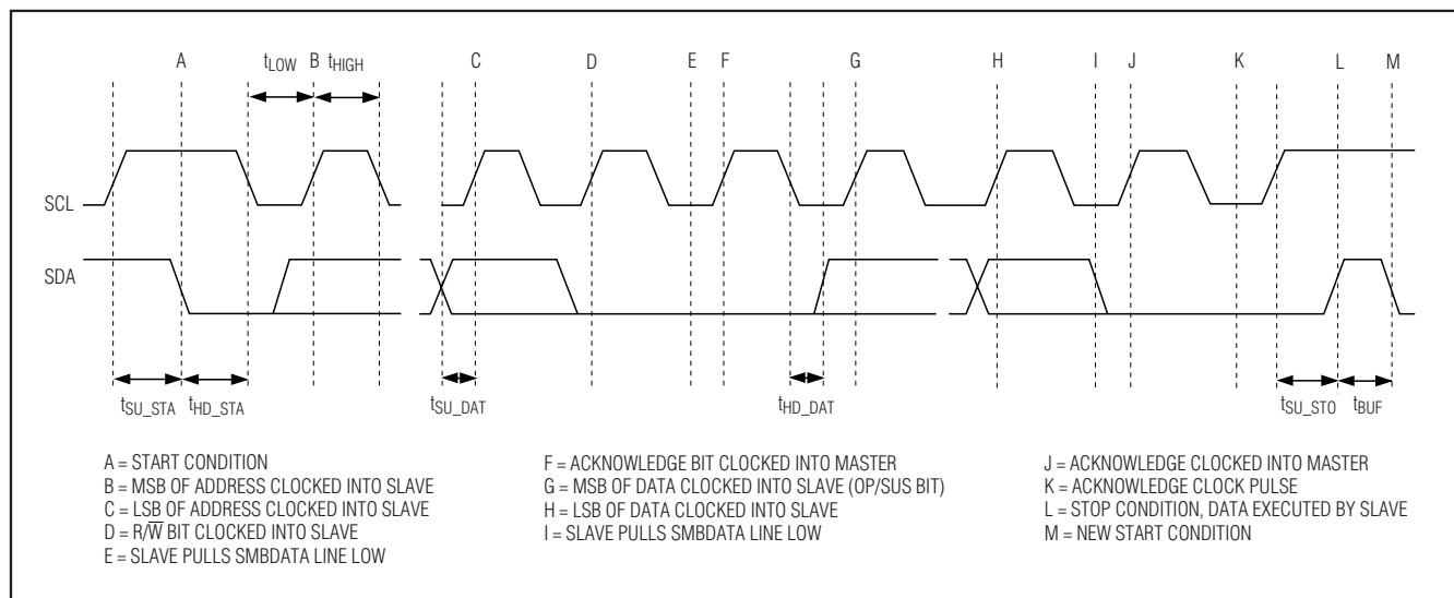
Figure 8. I²C Timing Diagram
