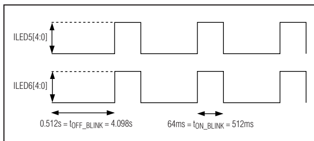
Figure 5. Blink Timer Behavior
