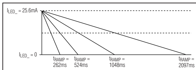
Figure 4. Ramp-Down Behavior
