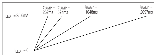
Figure 3. Ramp-Up Behavior
