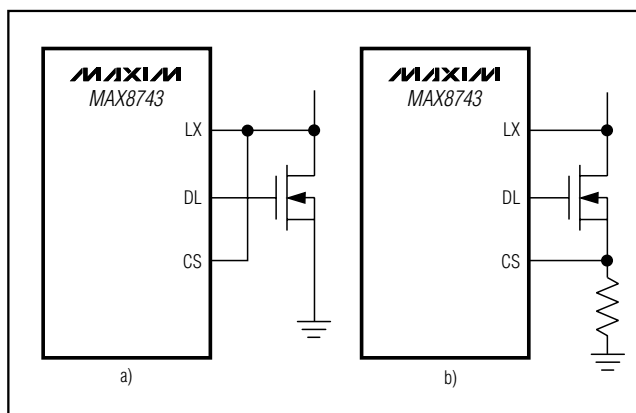
Figure 7. Current-Sense Configurations
