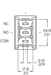
Single Pole
