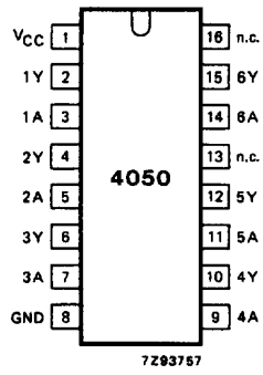
Fig.1 Pin configuration.
