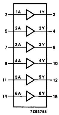
Fig.2 Logic symbol.
