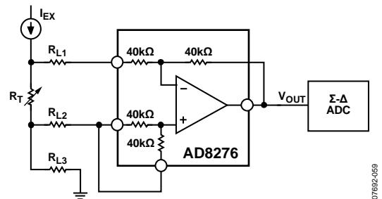
Figure 53. 3-Wire RTD Cable Resistance Error Measurement
