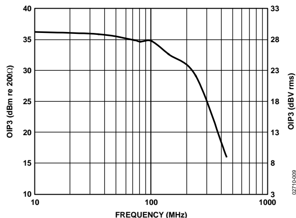
Figure 9. OIP3 vs. Frequency for V_{GAIN} = 500 mV
