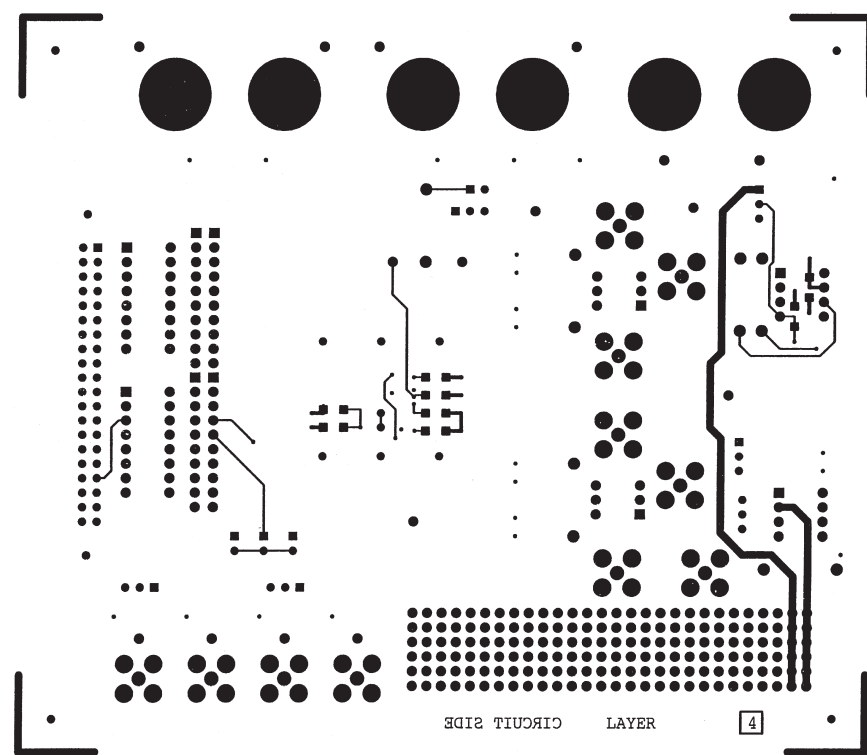
Figure 29. Solder Side PCB Layout (Layer 4)
